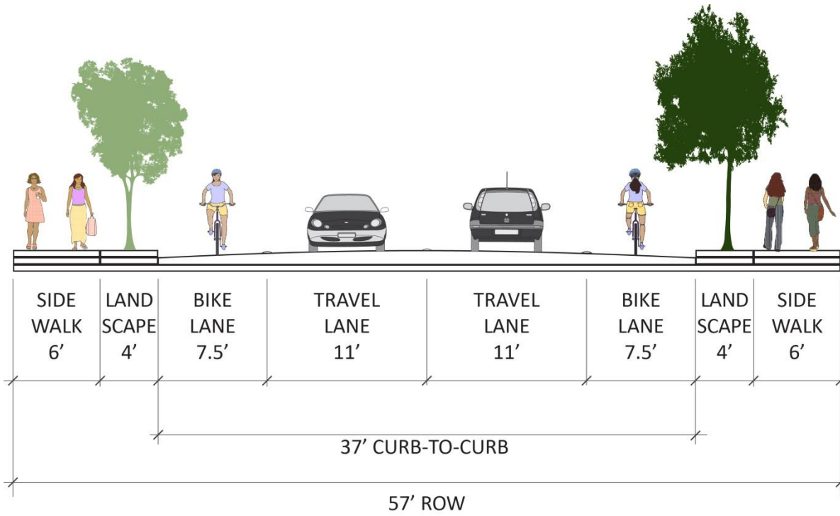
Figure 24. Traditional Section
